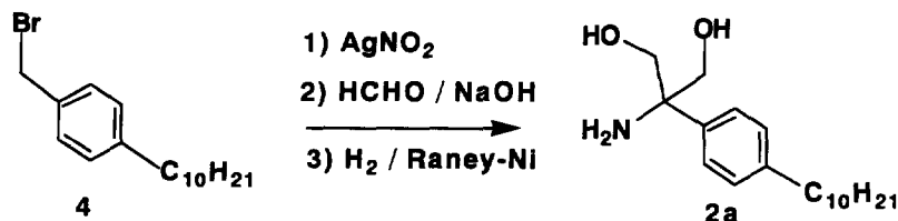
Scheme 2. Synthesis of 2a .
